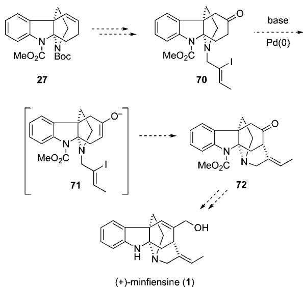
Scheme 16
