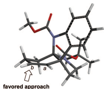
Figure 3. Proposed rationale for stereoselection in the epoxidation of alkene 27. Model (6-31G*) of the most stable conformation of alkene 27 showing the favored approach of an oxidant to alkene carbon b .
