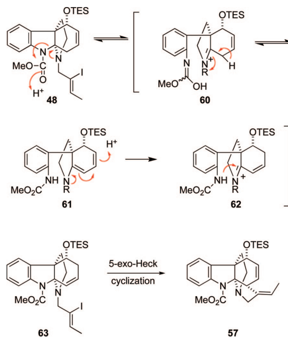
Scheme 12
