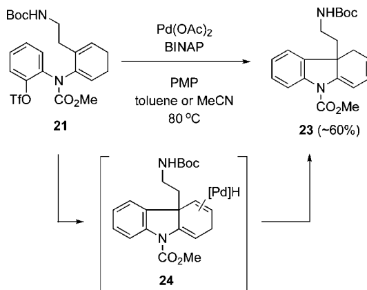
Scheme 4
