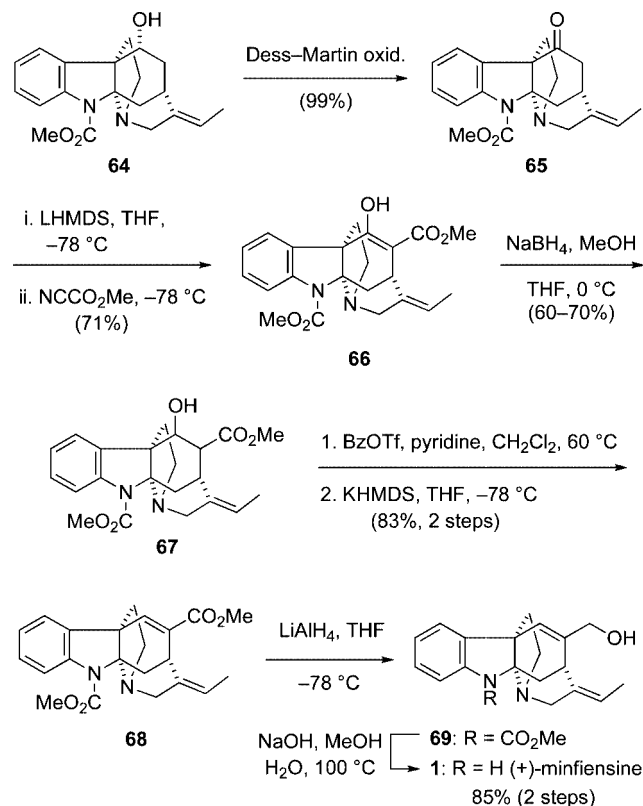
Scheme 14
