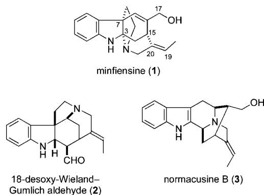
Figure 1. Minfiensine ( 1 ) and two additional C 19 H 22 N 2 O Strychnos alkaloids.
