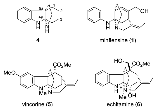
Figure 2. Representative alkaloids containing a 1,2,3,4-tetrahydro-9a,4a-(iminoethano)-9H-carbazole.
